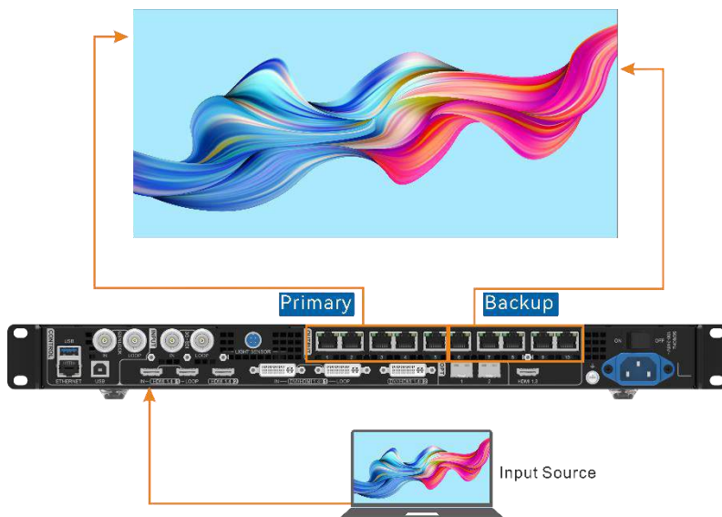
Figure 5-27 Ethernet port backup connection
