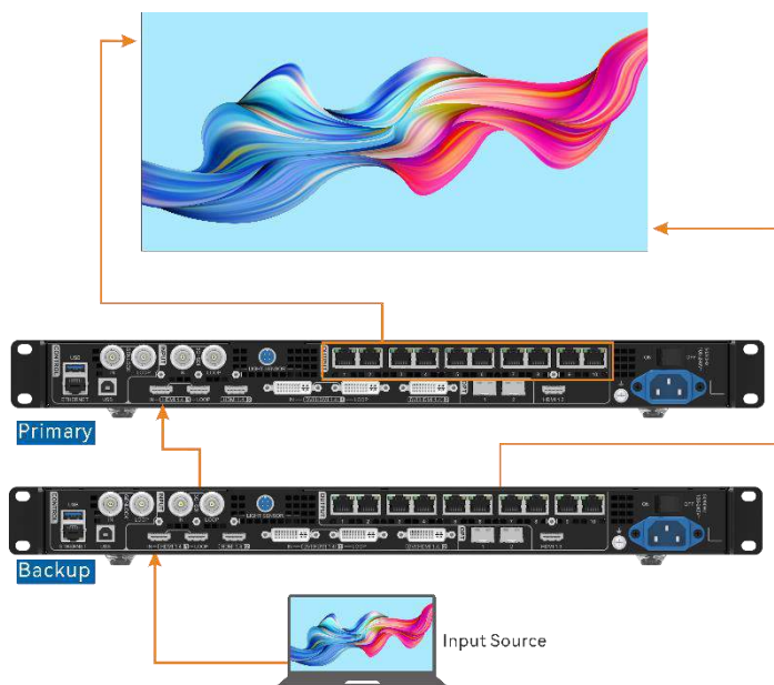
Figure 5-25 Device backup connection
