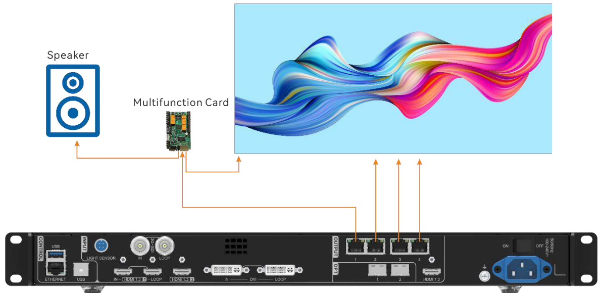
Figure 5-35 Audio output connection
