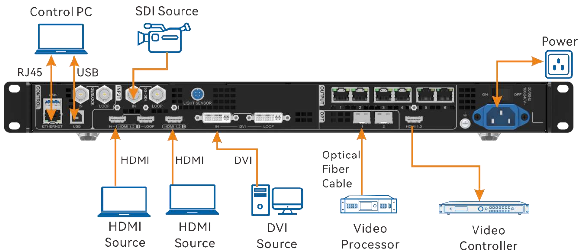
Figure 5-33 HDMI output
