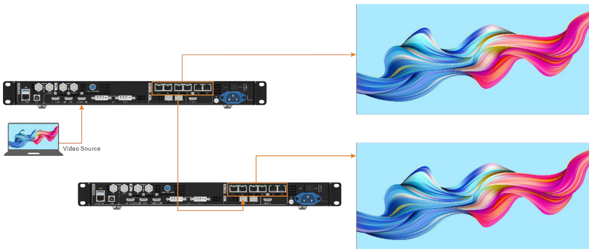
Figure 5-39 Copy
