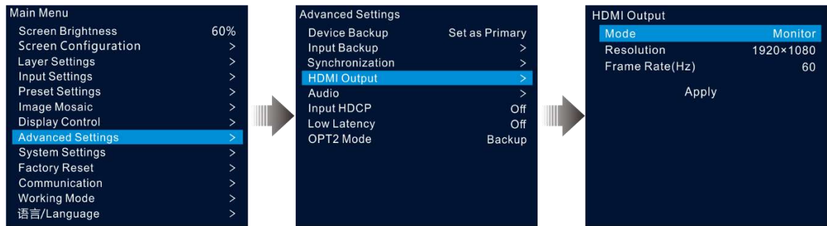
Figure 5-34 HDMI output
