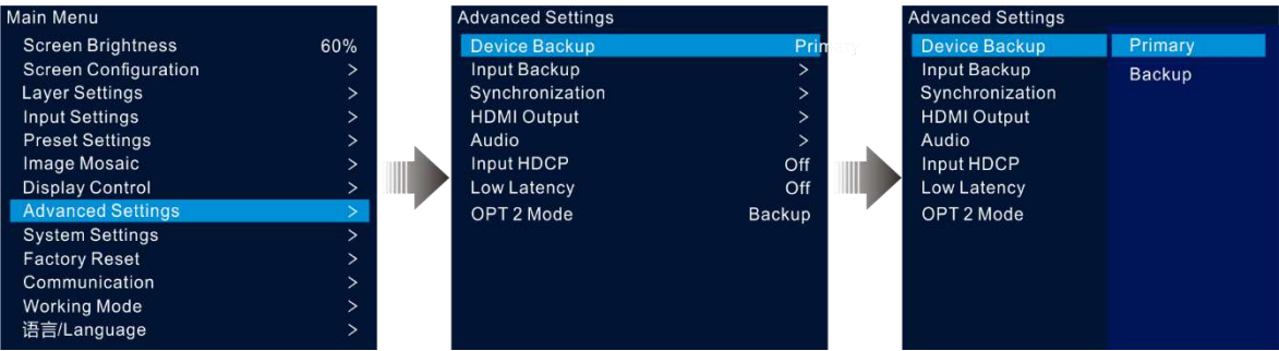
Figure 5-26 Device Backup
